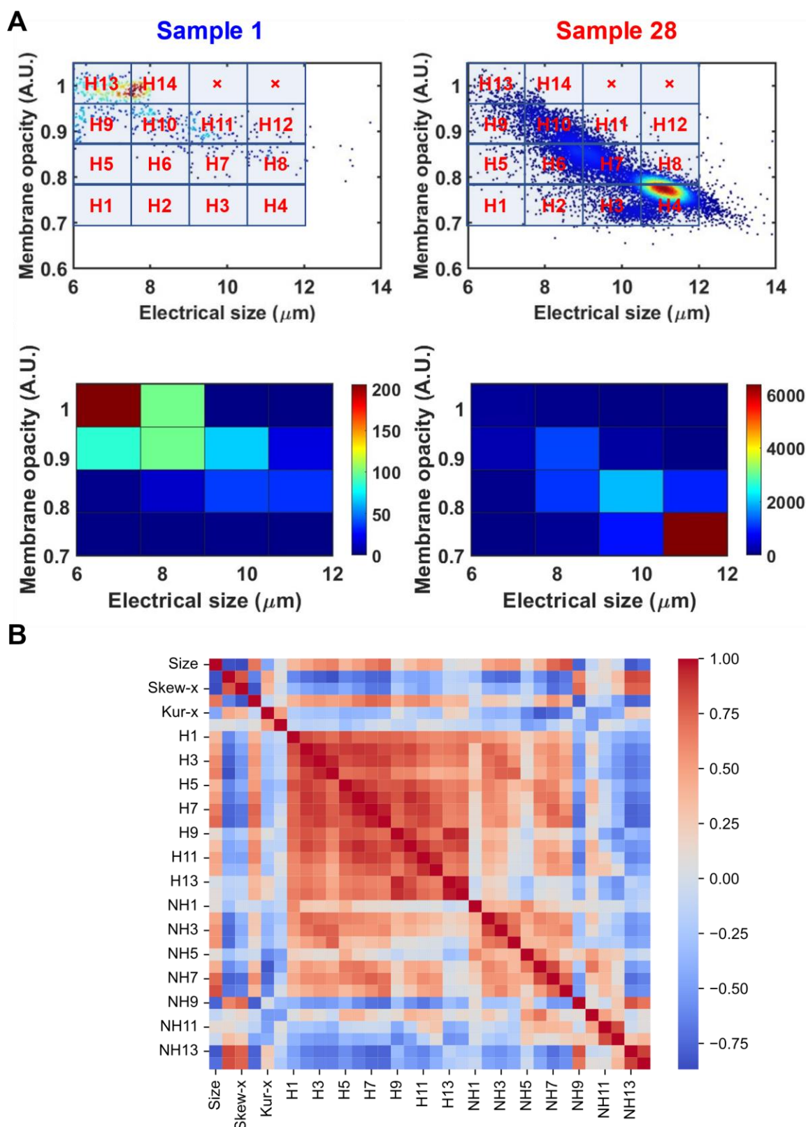
Figure S9 Feature definition and analysis. (A) bivariate histogram features of representative impedance profiles. Overlaid histogrambins on impedance profile (top) and tile bivariate histogram with cell count as color (bottom). × regions were excluded from the analysis as they correspond to reference bead population. (B) Correlation of 34D impedance features
